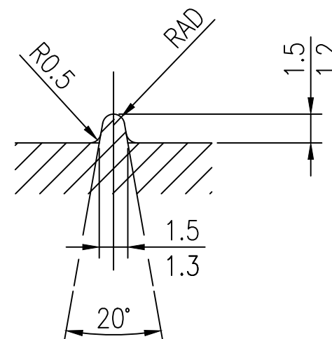
BRANDING PROFILE FOR LETTER 'C' & 'D' SCALE 4 : 1
